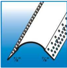
Roh Bullnose Outside Corner Bead
