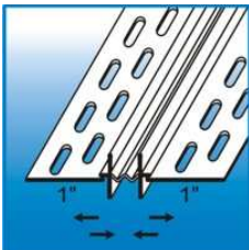
Hideaway Expansion 3,05 m
